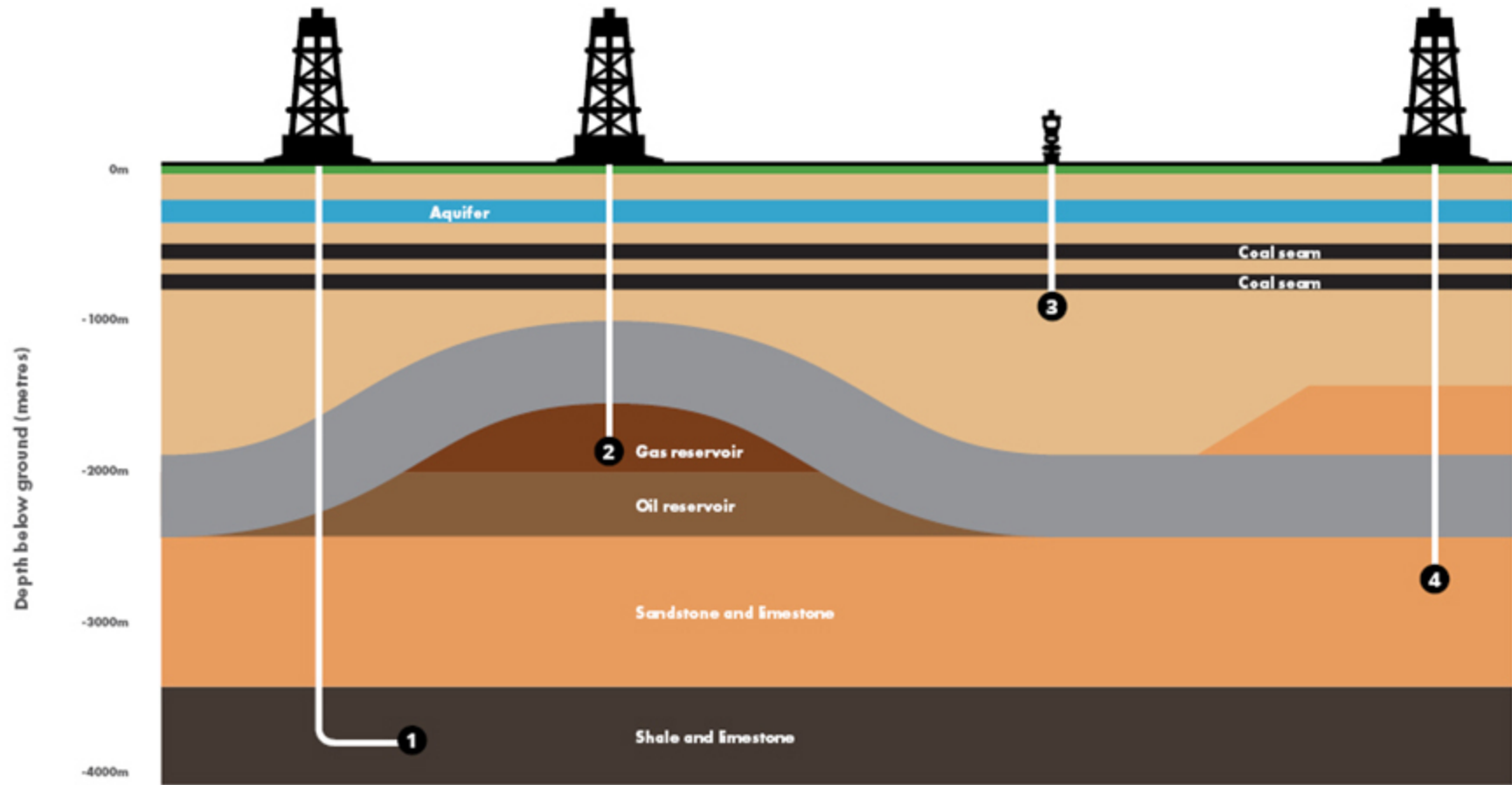
1. Shale gas well 2. Conventional well 3. Coal seam gas well 4. Tight gas well
